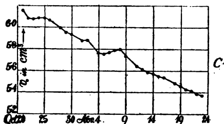
FIG. 19, A, B, C.—Chart showing loss of standard volumes of gas in diver in lapse of days. Diffusion of air through water.
